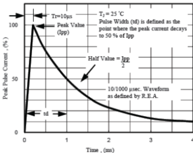
Fig. 5 - Pulse Waveform
