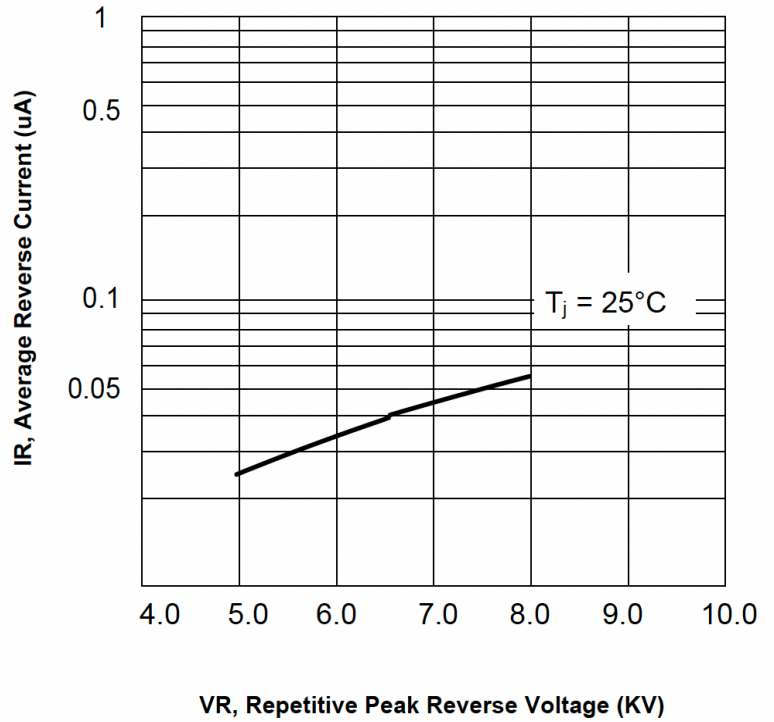
REVERSE CHARACTERISTIC
