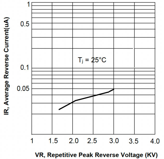
REVERSE VOLTAGE CHARACTERISTIC DISTRIBUTION
