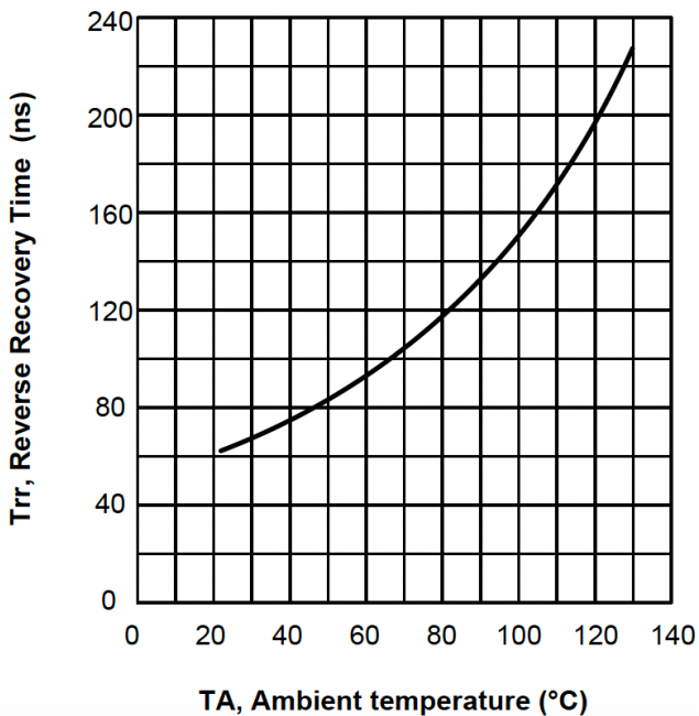
REVERSE RECOVERY TIME CHARACTERISTIC
