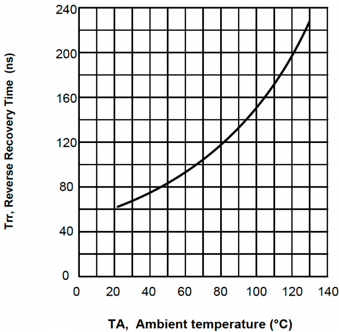
REVERSE RECOVERY TIME CHARACTERISTIC
