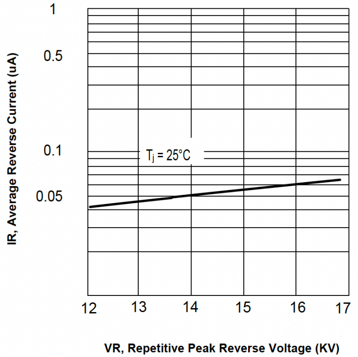
REVERSE VOLTAGE CHARACTERISTIC DISTRIBUTION
