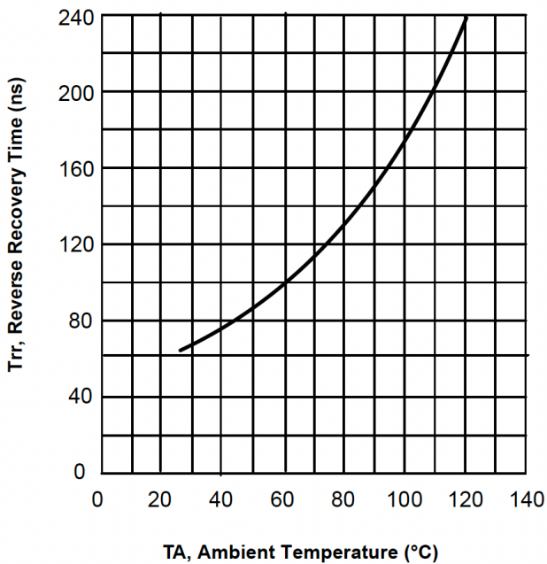
REVERSE RECOVERY TIME CHARACTERISTIC
