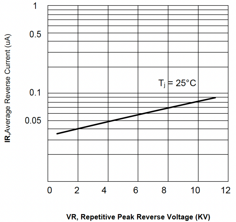
REVERSE CHARACTERISTIC
