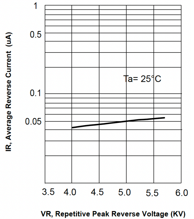
REVERSE CHARACTERISTIC
