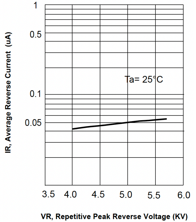
REVERSE CHARACTERISTIC
