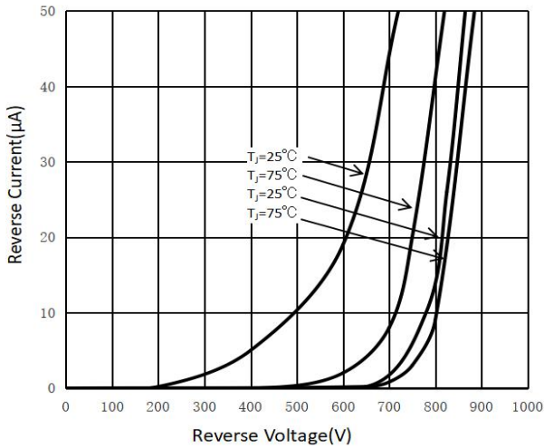
FIG.3: Reverse Characteristics
