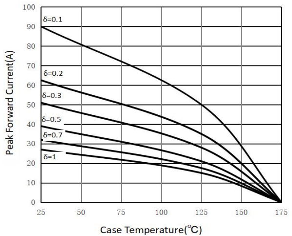
FIG.6: Current Derating
