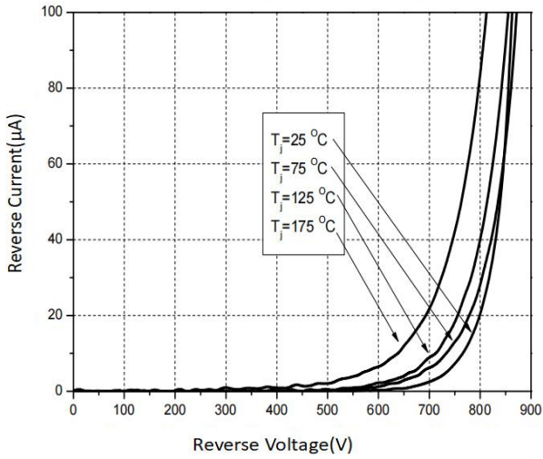
FIG.3: Reverse Characteristics
