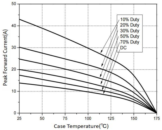
FIG.6: Current Derating
