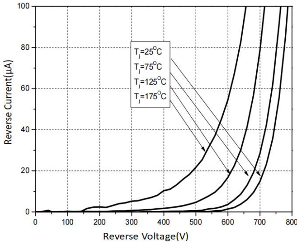
FIG.3: Reverse Characteristics
