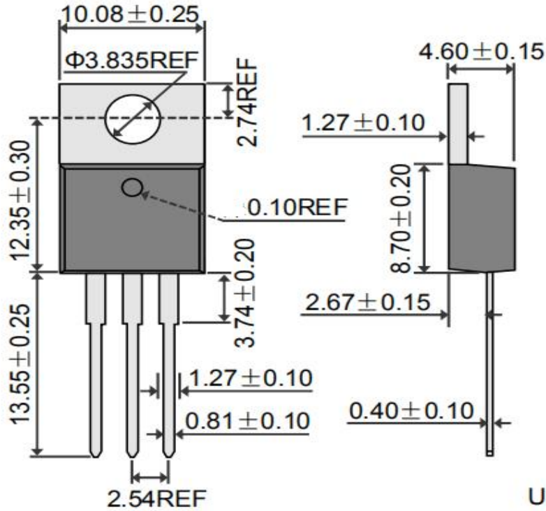
TO-220AB
